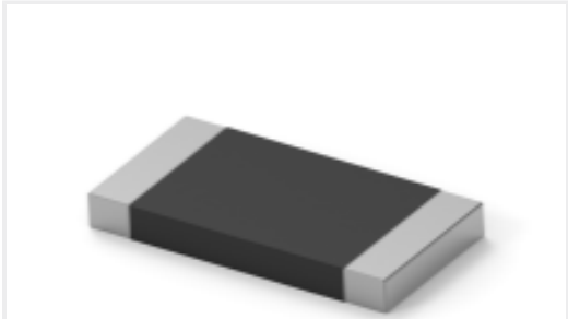
TE Part #6-2176422-6 TLRP 2512 3.0W R047 1% 50PPM 4K RL
