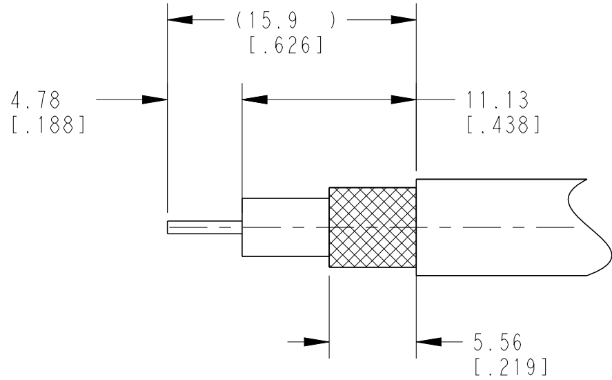
RECOMMENDED STRIP LENGTH SCALE 3:1
