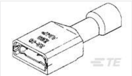
TE Part #2-520181-4 ULTRA-FAST 187 ASY REC 22-18 TPPB
