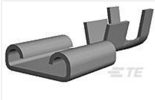
TE Part #42437-5 250 FASTON REC 14-10 AWG TPBZ
