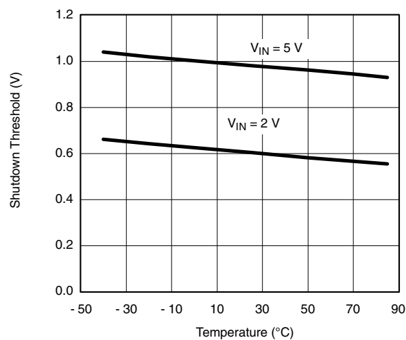
Shutdown Threshold vs. Temperature
