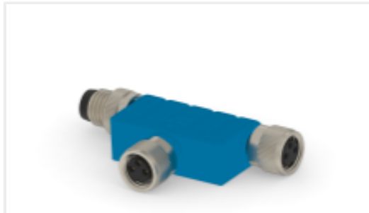
TE Part #T4082102003-000 M8 T DISTRIBUTOR MALE 3POS
