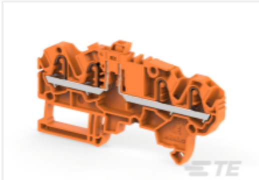
TE Part #1SNK705331R0000 ZK2.5-S-4P-OR
