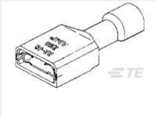
TE Part #3-520150-2 ULTRA-FAST 187 ASY REC 16-14 AWG TPBR
