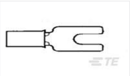
TE Part #41495 SPADE .190(4.82 MM)12-10 AWG TPBR
