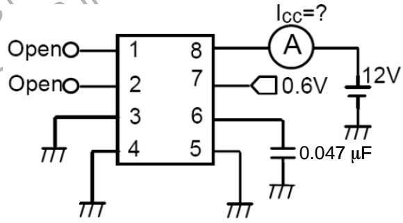
Figure 16. Supply Current 2
