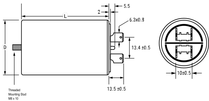
Double Faston
