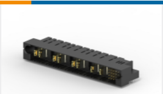
TE Part #1892302-1 MBXL R/A HDR DB 11P+12S
