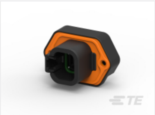
TE Part #DTP15-4P HDR, 4P, BLK, ST, SN/NI/CU
