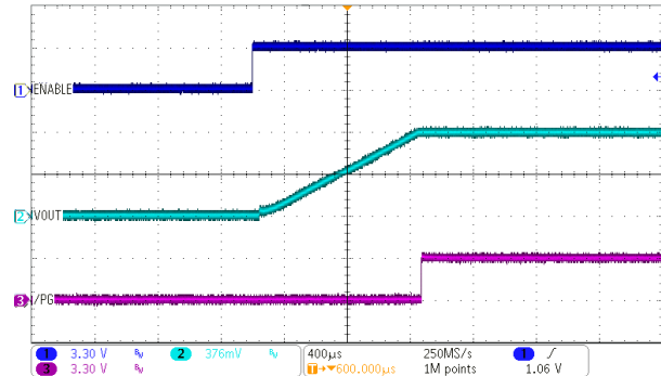
Load = 0.75\Omega Figure 10-21. Start-Up Using the EN Pin
