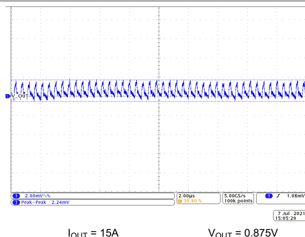
Figure 10-13. Output Voltage Ripple
