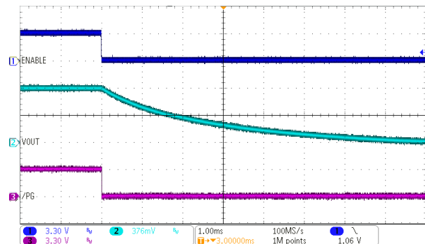
Load = 7.5\Omega Figure 10-23. Shutdown (Discharge disabled)
