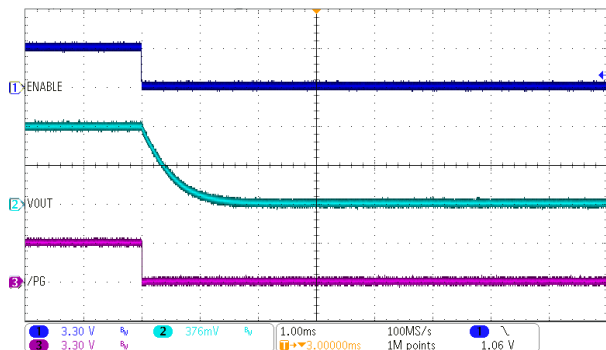
Load = 7.5\Omega Figure 10-22. Shutdown Using the EN Pin (Discharge Enabled)
