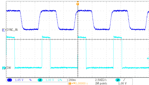
Load = 0.75\Omega FSEL = 2.25MHz f_{(\text{SYNC})} = 2MHz Figure 10-20. Synchronization to an External Clock
