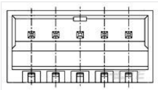
TE Part #5-1775444-6 EMIX CONN., 1.5MM PITCH, HDR, R /A, 6P
