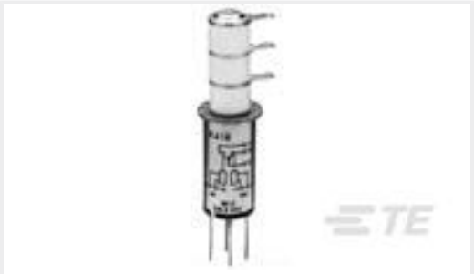
TE Part #7-1618239-7 K41R332=RELAY, VACUUM, SPDT
