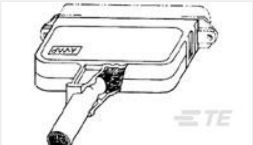
TE Part #552008-1 KIT, COVER, 180, 50 POS
