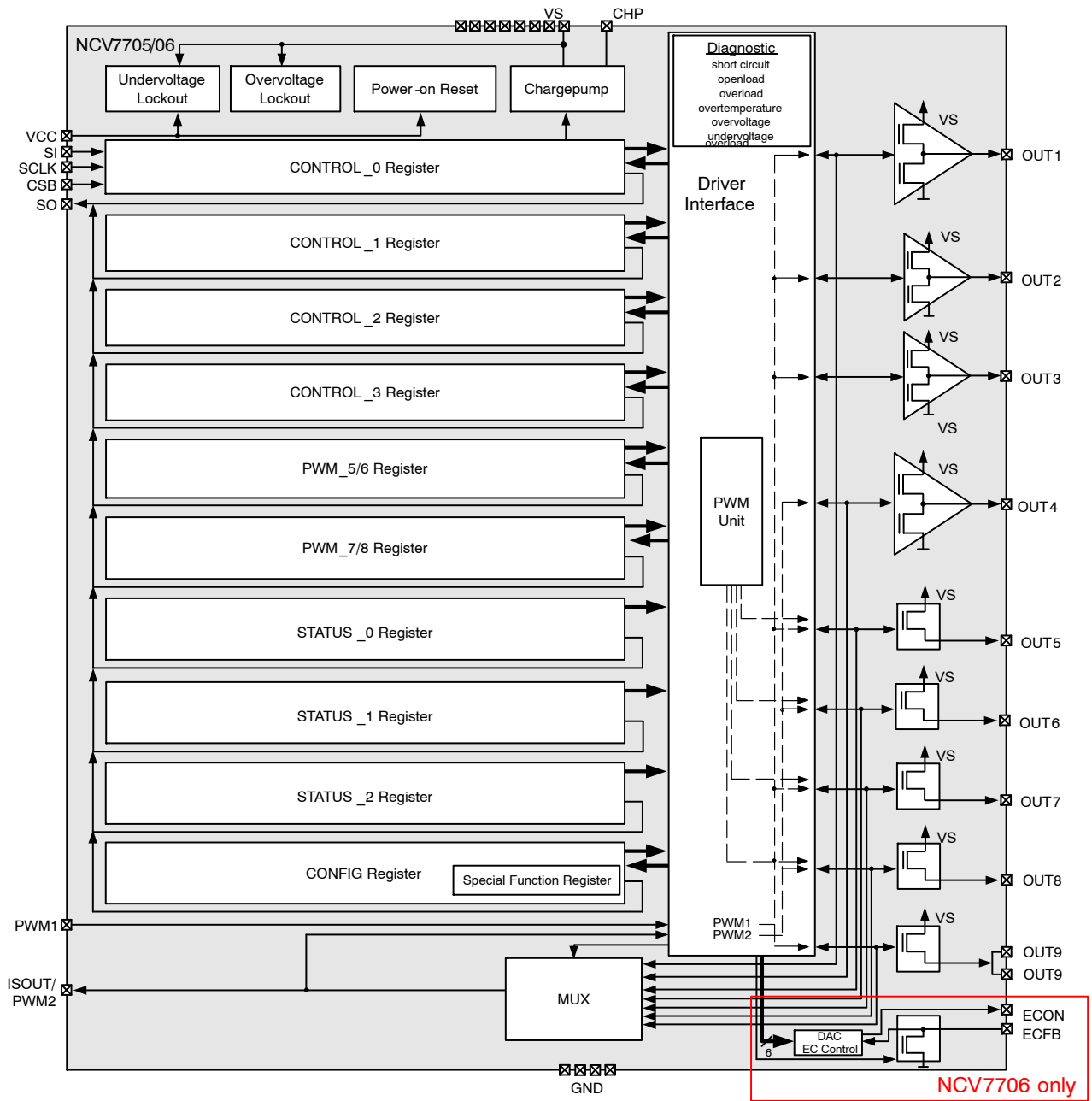
Figure 1. Block Diagram
