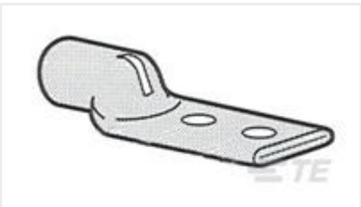
TE Part #326803 TERM, AMPPOWER, 4/0, 3/8, 2 HOLE
