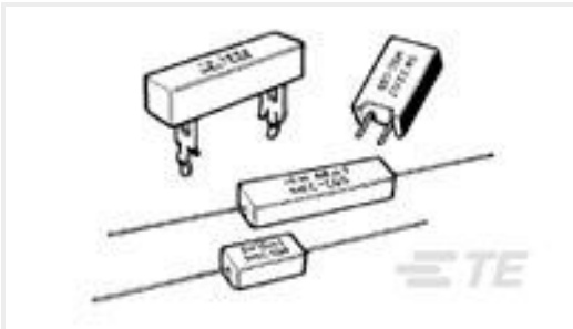
TE Part #1623782-8 SQM5 2K2 5% (METAL FILM)
