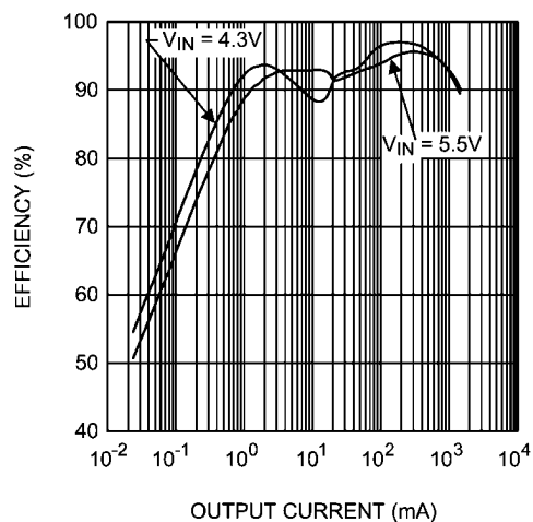
Buck 2 Efficiency vs Output Current (PFM to PWM Mode, V_{out} = 3.3V , L = 2.2\mu H )
