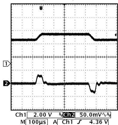
Line Transient (LDO1) 3.6 - 4.5\text{V}_{in} , 3.3\text{V}_{out} , 150 mA load
