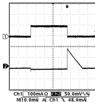
Load Transient (LDO2) 3.6\text{V}_{in} , 1.8\text{V}_{out} , 0 – 100 mA load
