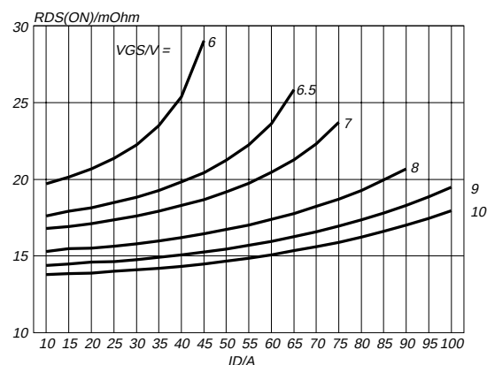
Fig.6. Typical on-state resistance, T_j = 25\text{ °C} . R_{DS(ON)} = f(I_D) ; parameter V_{GS}
