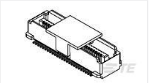
TE Part #1759898-1 0.6 BTB 50 Posn MH_5.5 Plug
