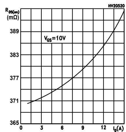
Figure 6. Typical drain-source on-resistance
