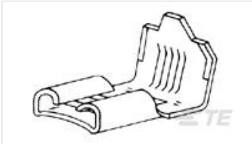
TE Part #62057-3 250 FASTON FLAG REC 12-10 AWG TPBR
