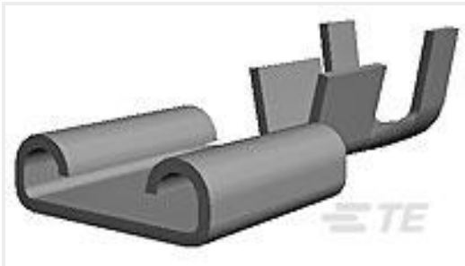
TE Part #180363-2 250 FASTON,REC.,12-10 AWG,TPBR
