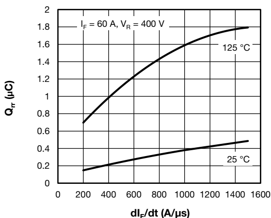
Fig. 8 - Diode Reverse Recovery Charge vs. dl_F/dt
