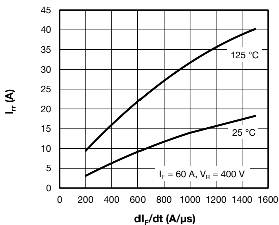
Fig. 7 - Diode Reverse Recovery Current vs. dl_F/dt
