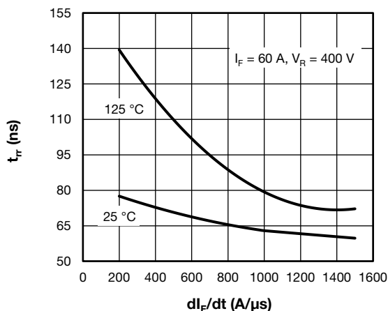
Fig. 6 - Diode Reverse Recovery Time vs. dl_F/dt
