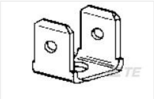
TE Part #61914-1 187 FASTON TAB PBR
