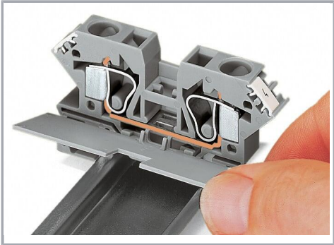
Snapping a cover plate onto open side of terminal block.
