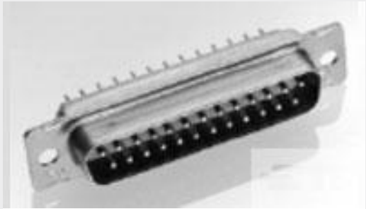
TE Part #1757819-4 AMPLIMITE,ASY,PLUG,STD,109,ZN,4
