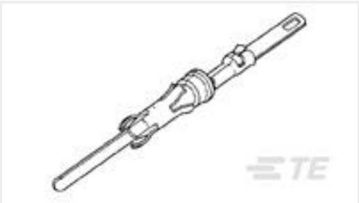
TE Part #202236-1 III+ PIN,SOLTAB,30AU,10AU FLASH,LP
