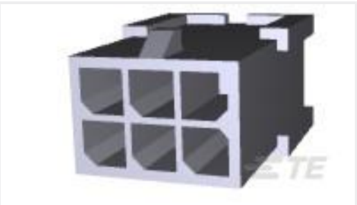
TE Part #794616-6 FREE HANG DBL ROW HSG 6 POS
