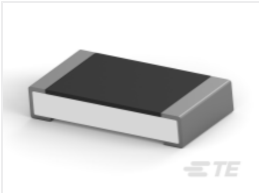
TE Part #2-2176388-3 RQ 1206 16R9 0.1% 10PPM 5K RL
