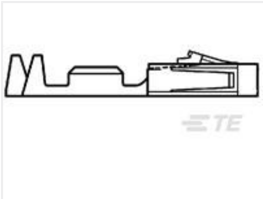
TE Part #1-104479-0 SHORT POINT CONT 30 DPLX STMPD LF
