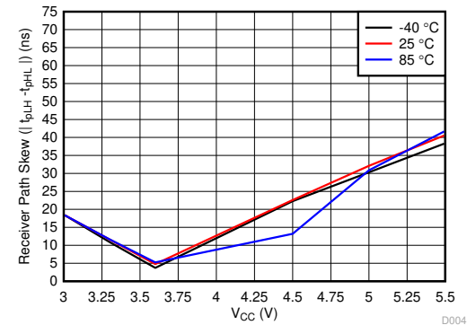
D004_rx_skew.grf
