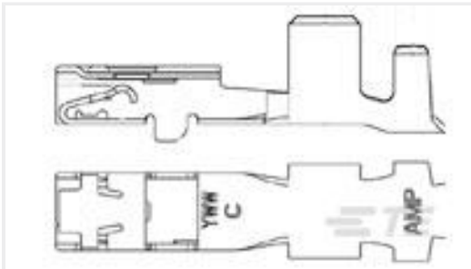
TE Part #1326030-2 2.8MM RECPT,UNSEAL,18-20AWG
