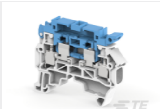
TE Part #1SNK508419R0000 ZS4-S-R3-T2
