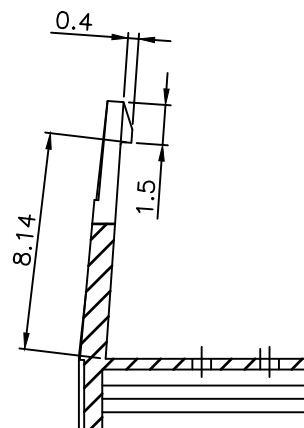
SECTION Z-Z
