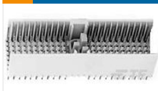
TE Part # 6645141-1 2MM H.M. 8 + 2 ROW TYPE "F" PI
