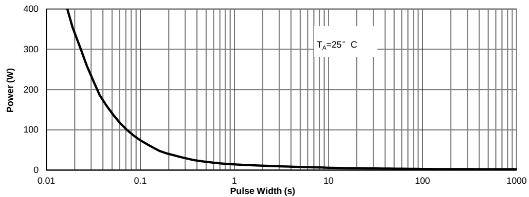
Figure 14: Single Pulse Power Rating Junction-to-Ambient (Note G)
