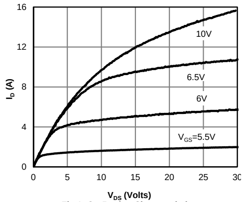
Fig 1: On-Region Characteristics
