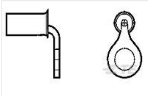
TE Part #322768 TERMINAL,SOLIS R 90DEG 22-16
