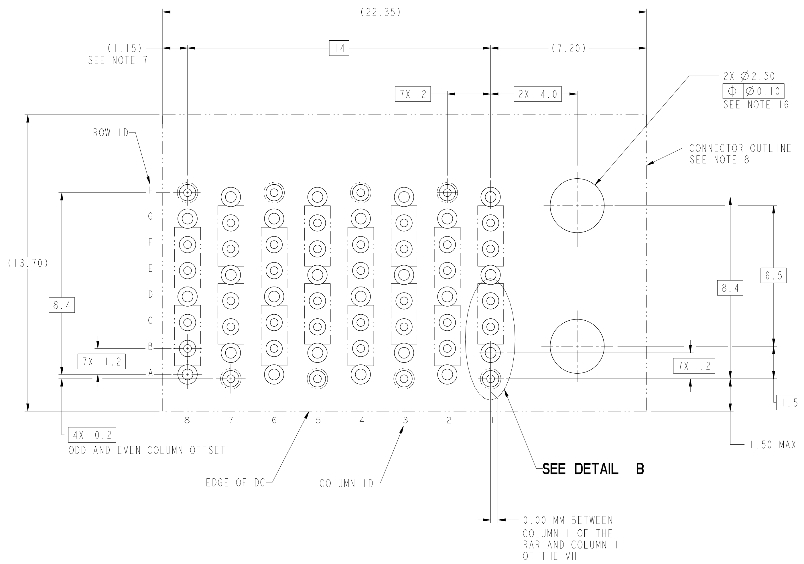
10124411-X1AYLF THRU -X1JYLF RECOMMENDED PCB LAYOUT COMPONENT SIDE NOTES 7, 8, 9, 11 & 16 SCALE 10:1
