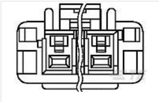
TE Part #1376393-1 5MM POWER KEY 6P PLUG HSG NUT
