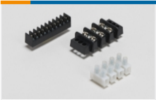
Barrier Strips(41)
