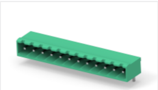
TE Part #1-2350513-2 12POS TB HDR 90 DEG, PITCH 5.0 & TL 4.5mm
