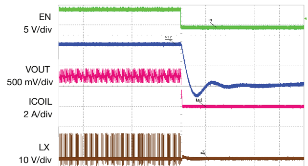
Fig. 17 - Shut-Down, I_{OUT} = 3\text{ A} , Time = 50 μs/div
