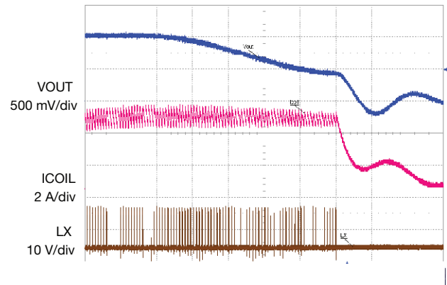
Fig. 18 - Over Current Protection, I_{VALLEY} = 4\text{ A} , Time = 20 μs/div
