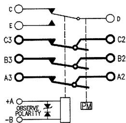
Circuit Configuration 18
