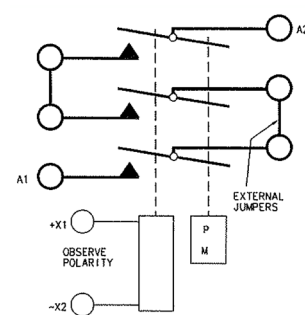
Circuit Configuration 12
