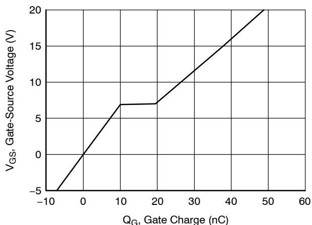
Figure 8. Typical Gate Charge at V_{DS} = 800\text{ V} and I_D = 25\text{ A}
